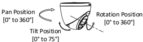
Figure 2-21 3-Axis Adjustment
