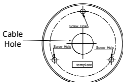
Figure 2-1 Drill Template
