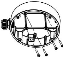
Figure 2-26 Secure Junction Box Body
