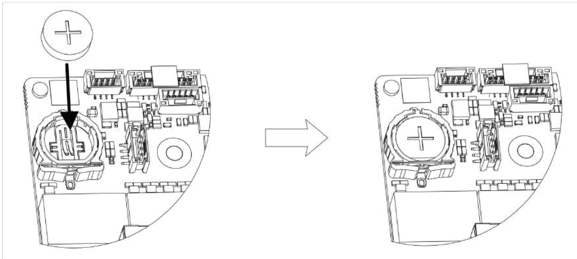
Figure 1-2 Replace Battery
