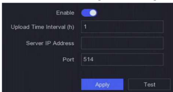
Figure 6-7 Log Server Settings
