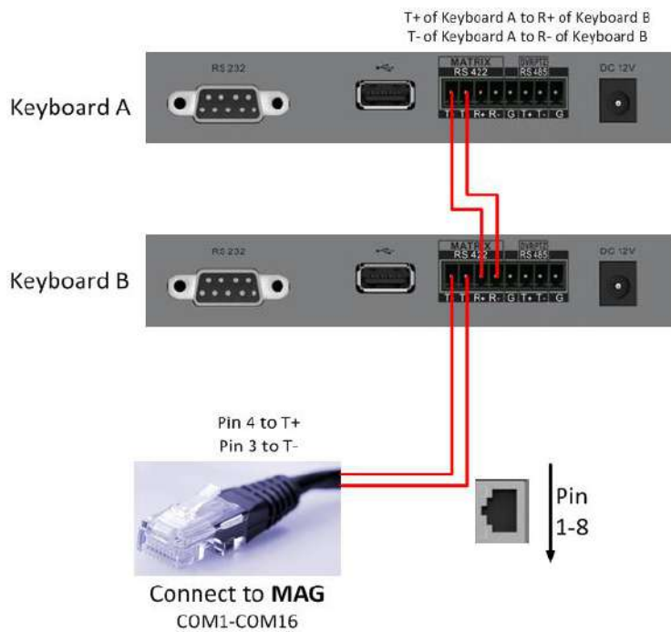
Figure 3-7 Connection between Cascaded Keyboards and MAG
