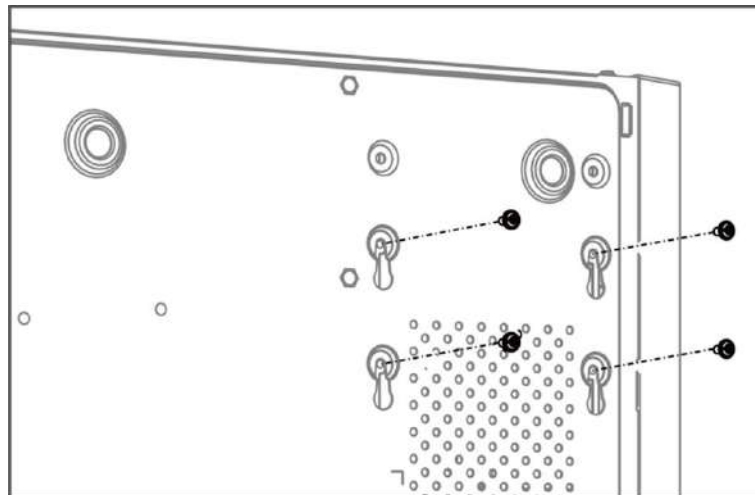
Figure 1-11 Fix HDD to Device Bottom
